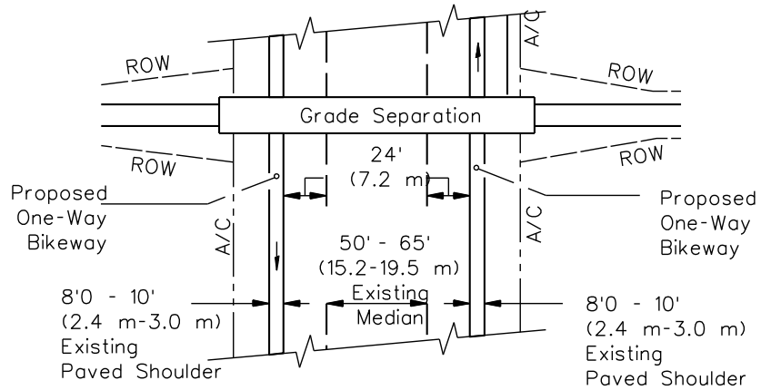
PLAN VIEW OF ONE-WAY BIKEWAY UNDER BRIDGE
