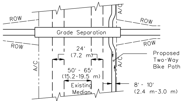
PLAN VIEW OF TWO-WAY BIKE PATH UNDER BRIDGE
